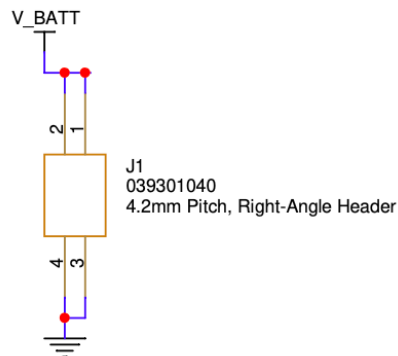
Figure 12.2: Battery Mux: Battery in Power out Schematic.
