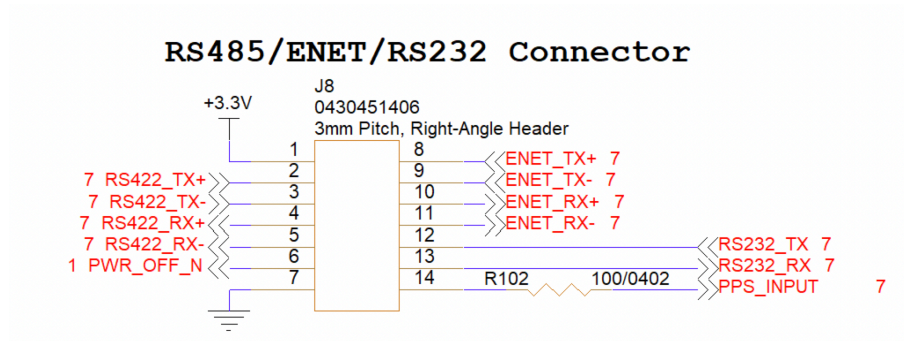
Figure 11.2: PDI Schematic connections.
