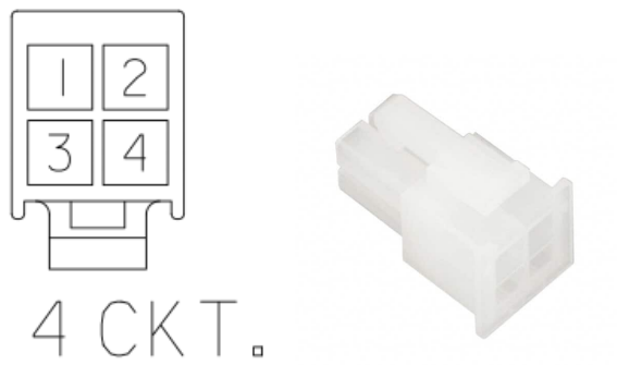
Figure 12.3: PMM5021 Power Connectors and pinout.
