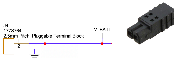
Figure 11.6: PMM3511 Power Connectors and pinout.
