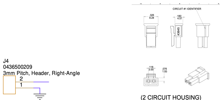
Figure 11.7: PMM3511 Rev 40+ Power Connectors and pinout.
