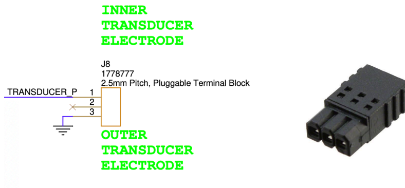
Figure 11.9: PMM3511 Transducer connector and pinout for board revisions 00-30.
