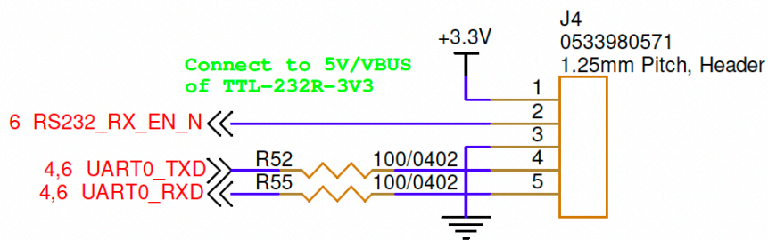
Figure 11.3: Popoto TTL Uart Plug. This port allows 3.3V Logic level uart connections
