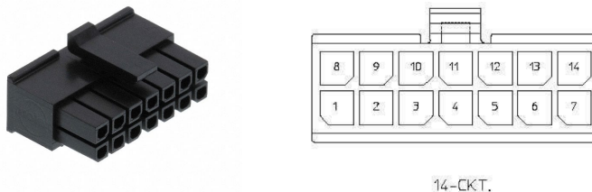
Figure 11.1: PDI User-Side Molex Connector. Interfacing to the PDI is accomplished with a Molex Microfit shell P/N 0430251400 and either Pre-pinned jumper wires, or Molex socket crimps.
