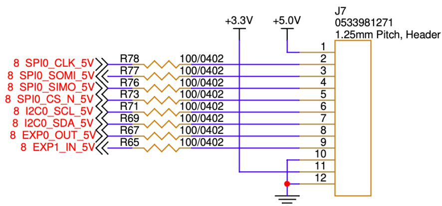
Figure 11.4: Popoto Expansion Header. This connector allows access to I2C, SPI and General purpose I/O from the Popoto Modem.
