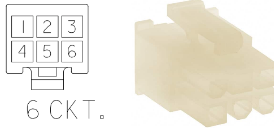
Figure 15.10: PMM5021 Transducer connector and pinout.
