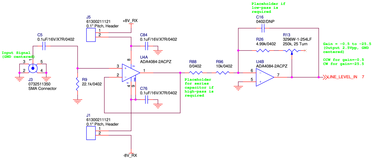
Figure 15.11: PMM5021 Analog input schematic excerpt. This circuit conditions the input signal and is used for SSB voice input or for applications providing line level analog input.
