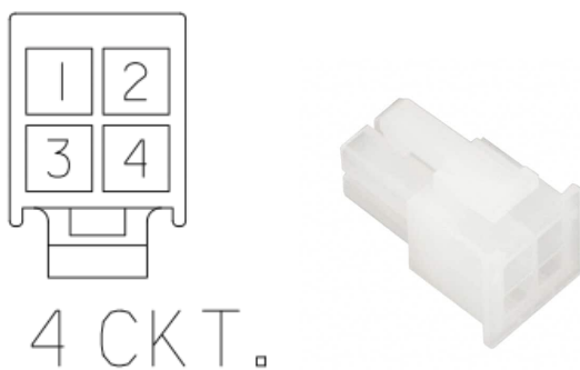
Figure 15.7: PMM5021 Power Connectors and pinout.
