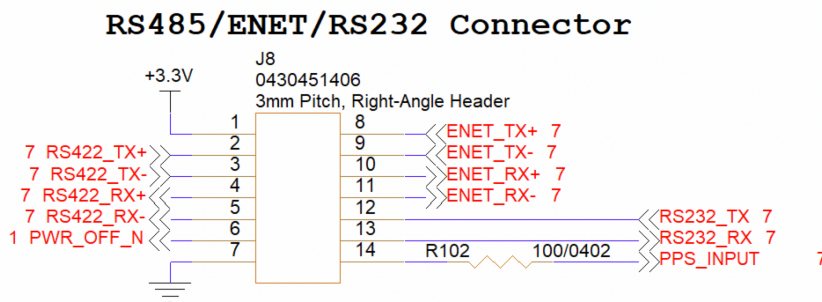
Figure 15.2: PDI Schematic connections.
