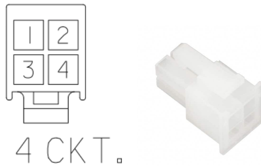
Figure 13.7: PMM5021 Power Connectors and pinout.
