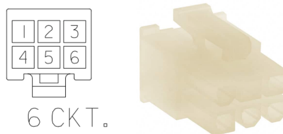
Figure 13.10: PMM5021 Transducer connector and pinout.
