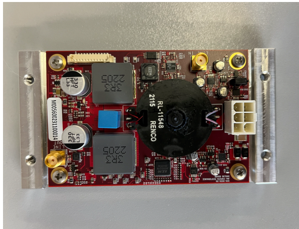
Figure 2.1: The PMM5021 Analog board
