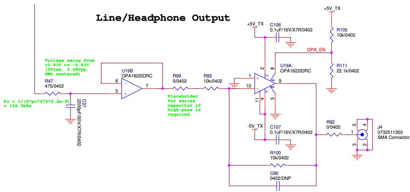
Figure 13.12: PMM5021 Analog output schematic excerpt. This circuit provides a +/- 5V signal to the SMA output port. This signal is used for the headphones output during SMA voice mode, or for a diagnostic port or to drive an external power amplifier if needed.
