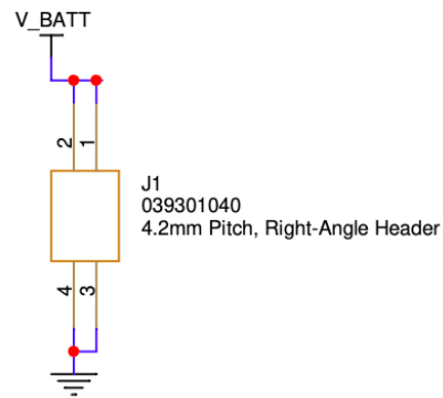
Figure 13.6: PMM5021 Power Schematic.
