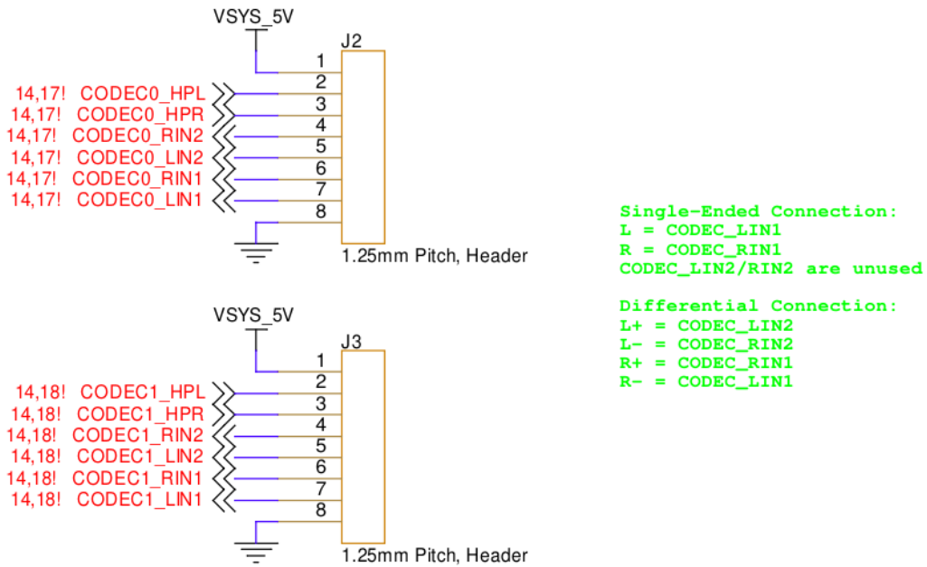
Figure 15.9: The additional inputs and outputs on the PMM5544
