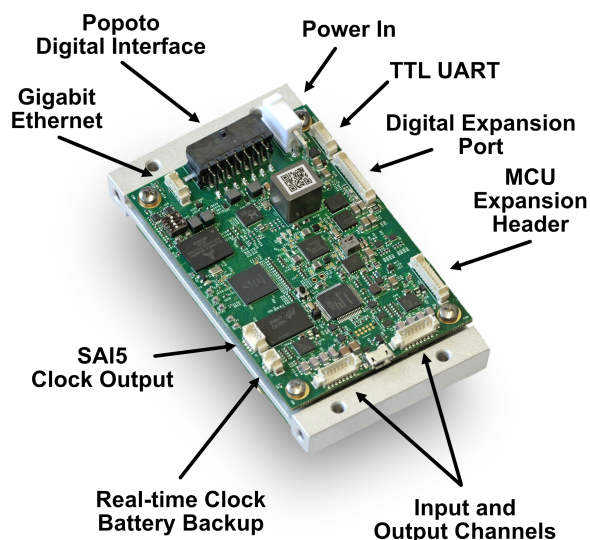
Figure 15.6: PMM5544 Digital Board Connector Locations
