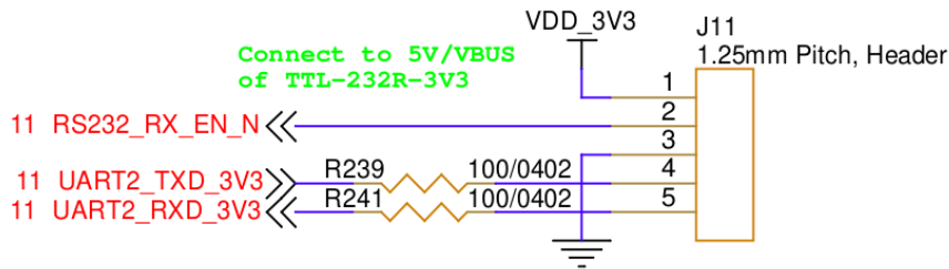
Figure 15.3: Popoto TTL UART Plug. This port allows 3.3V logic-level UART connections
