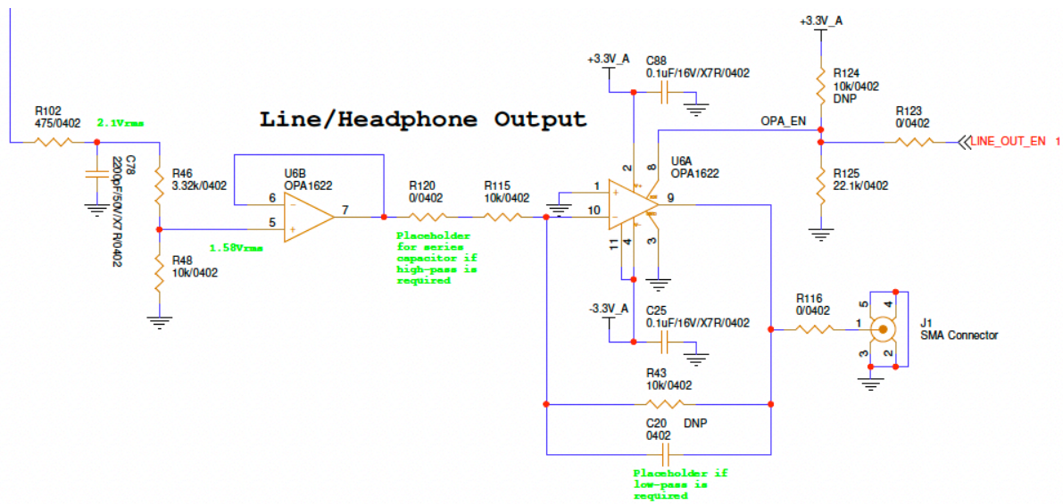
Figure 15.14: PMM5544 Analog output schematic excerpt. This circuit provides a +/- 3.3V signal to the SMA output port. This signal is used for the headphones output during SMA voice mode, or for a diagnostic port or to drive an external power amplifier if needed.
