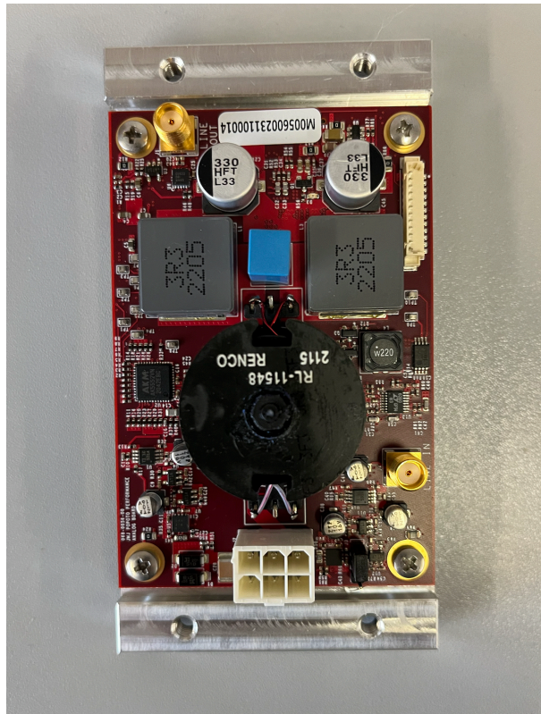
Figure 15.10: The PMM5544 Analog board
