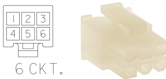
Figure 15.12: PMM5544 Transducer connector and pinout.
